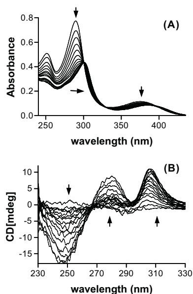
Figure 4. DNA titration of 28a followed by (A) absorption and (B) circular dichroism spectroscopies. To 1 mL of drug solution at 20 \mu\text{M} were added aliquots of a concentrated calf thymus DNA solution. The phosphate-DNA/drug ratio increased from 0 to 20. Measurements were performed in BPE buffer pH 7.1 (6 mM \text{Na}_2\text{HPO}_4 , 2 mM \text{NaH}_2\text{PO}_4 , 1 mM \text{Na}_2\text{EDTA} ). Spectra are referenced against DNA solutions of exactly the same DNA concentration and were adjusted to a common baseline.
