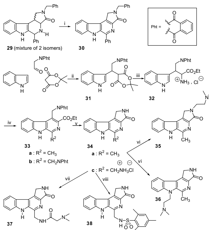
Scheme 7. Reagents and conditions: (i) TCCA, Et 3 N, rt, 83%; (ii) see Ref. 32, 73%; (iii) see Ref. 34, three steps, overall yield 39%; (iv) R 2 CHO, CH 2 Cl 2 , Et 3 N, TFA, molecular sieves 4 Å, then TCCA, Et 3 N, rt, 45–57%; (v) 34a : BuNH 2 , reflux, 90%; 34c : 6 M HCl solution, reflux, 78%; (vi) NaH, DMF, Cl(CH 2 ) 2 NMe 2 ·HCl, 17% ( 35 ) and 26% ( 36 ); (vii) Me 2 NCH 2 CO 2 H, Et 3 N, ClCO 2 - i -Bu, CH 2 Cl 2 , BuOH, 78%; (viii) mesitylenesulfonylchloride, Et 3 N, DMF, rt, 71%.
