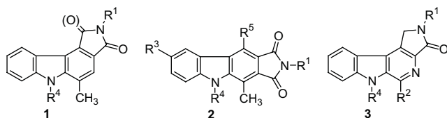
Scheme 1. 'Bended' and 'linear' pyrrolo-(aza)carbazoles.
