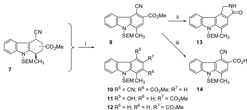
Scheme 4. Reagents and conditions: (i) activated \text{MnO}_2 , dry toluene, reflux, 9+10+11+12 (59%); (ii) \text{H}_2 , Raney-Ni, 6 bars, abs EtOH, dry toluene, rt, 94%; (iii) KOH (powdered), t -BuOH, toluene, \text{CH}_2\text{Cl}_2 , \text{H}_2\text{O} , 80 °C, 86%.
