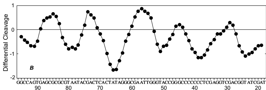
Figure 2. Differential cleavage plots comparing the susceptibility of the 176-bp DNA fragment to DNase I cutting in the presence of 50 \mu\text{M} 28a . Negative values correspond to a ligand-protected site and positive values represent enhanced cleavage. Vertical scales are in units of \ln(\text{fa}) - \ln(\text{fc}) , where fa is the fractional cleavage at any bond in the presence of the drug and fc is the fractional cleavage of the same bond in the control, given closely similar extents of overall digestion. Each line drawn represents a 3-bond running average of individual data points, calculated by averaging the value of \ln(\text{fa}) - \ln(\text{fc}) at any bond with those of its two nearest neighbors. Only the region of the restriction fragment analyzed by densitometry is shown.
