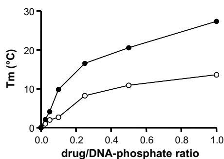
Figure 3. Melting temperature variation \Delta T_m ( T_m^{\text{drug-DNA complex}} - T_m^{\text{DNA alone}} in ^{\circ}\text{C} ) of poly(dAT) 2 (●) calf thymus DNA (○) after incubation with 28a . The T_m measurements were performed at increasing drug/DNA-phosphate ratio with a fixed DNA concentration (20 \mu\text{M} ). T_m measurements were performed in BPE buffer pH 7.1 (6 mM \text{Na}_2\text{HPO}_4 , 2 mM \text{NaH}_2\text{PO}_4 , 1 mM EDTA), in 1 cm quartz cuvettes at 260 nm with a heating rate of 1 ^{\circ}\text{C}/\text{min} . The T_m values were obtained from first-derivative plots.
