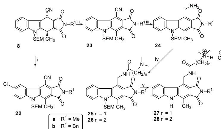
Scheme 6. Reagents and conditions: (i) TCCA, Et 3 N, dry DMF, rt, 26–36%; (ii) activated MnO 2 , dry toluene, reflux, 57–69%; (iii) H 2 , Raney-Ni, 6 bars, abs EtOH, dry toluene, rt, 52–70%; (iv) Me 2 NCH 2 CO 2 H, ClCO 2 - i -Bu, Et 3 N, CH 2 Cl 2 , BuOH, rt, 57% ( 25a ) and 37% ( 25b ) or Me 2 N(CH 2 ) n CO 2 H, DMTMM, MeOH, rt, 59–75% ( 25a , 26a and 26b ); (v) 3 M aq HCl solution, rt, 68–97%.
