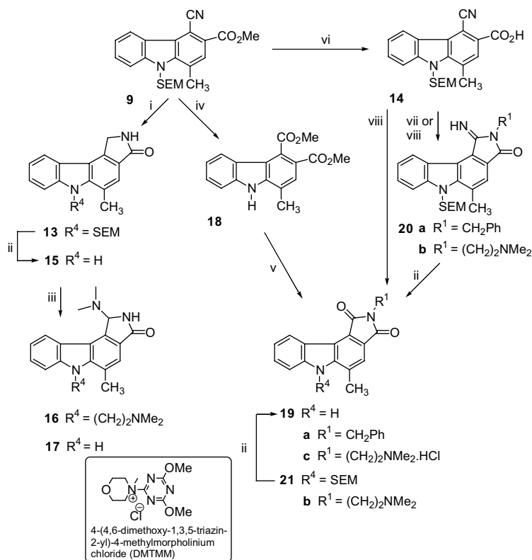
Scheme 5. Reagents and conditions: (i) \text{H}_2 , Raney-Ni, 6 bars, abs EtOH, dry toluene, rt, 94%; (ii) 3 M aq HCl solution, rt, 84–95%; (iii) NaH 50%, dry DMF, \text{Cl}(\text{CH}_2)_2\text{NMe}_2 \cdot \text{HCl} , rt, 23% ( 16–17 ); (iv) 9 M HCl/MeOH, reflux, 71%; (v) \text{H}_2\text{N}(\text{CH}_2)_2\text{NMe}_2 , 100 °C, 59%; (vi) KOH (powdered), t -BuOH, toluene, \text{CH}_2\text{Cl}_2 , \text{H}_2\text{O} , 80 °C, 86%; (vii) \text{H}_2\text{N}(\text{CH}_2)_2\text{NMe}_2 , \text{ClCO}_2 - t -Bu, \text{Et}_3\text{N} , \text{CH}_2\text{Cl}_2 , BuOH, rt, 28% ( 20b ); (viii) \text{R}^1\text{NH}_2 , DMTMM, MeOH, rt, 52% ( 21b )-83% ( 20a ).
