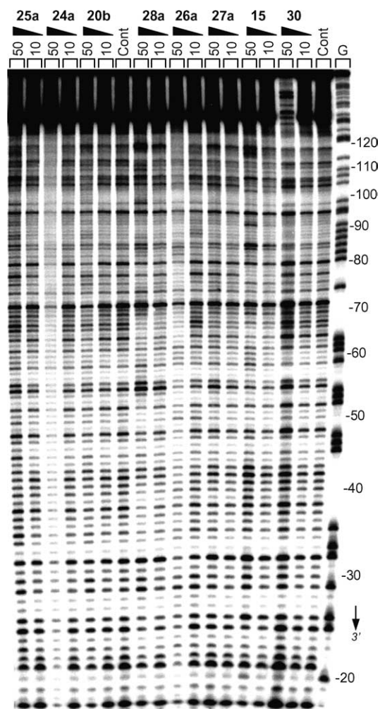
Figure 1. DNase I footprinting of 28a on a 3'-end radiolabelled 176-bp DNA fragment from pTUC. The products of nuclease digestion were resolved on an 8% polyacrylamide gel containing 8 M urea. The concentration in \mu\text{M} of the drug is shown at the top of the appropriate gel lanes. Control tracks (Cont.) contained no drug. The track labelled 'G' represents dimethylsulfate-piperidine markers specific for guanines.
