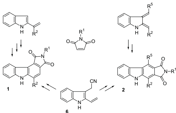
Scheme 2. Diels–Alder strategies towards 2,5-pyrrolidinedione-appended carbazoles 1 and 2 .
