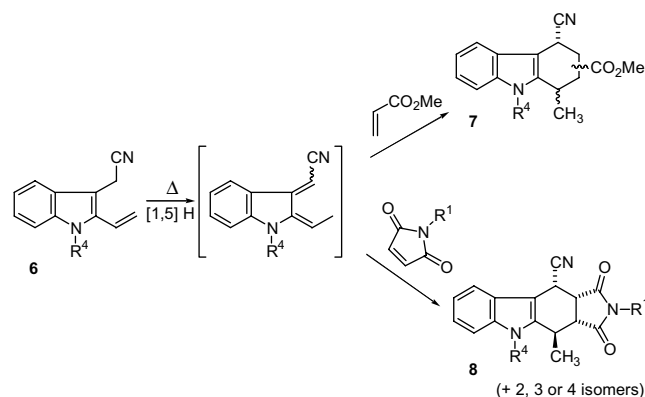
Scheme 3. Tandem [1,5]H sigmatropic shift/Diels–Alder reaction of 2-vinylindole 6 .
